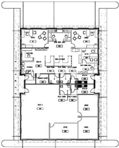
2 TENANT FIT-OUT FLOOR PLAN OPT. #2: BLDGS 1,3,4 & 6 1F-1 3000' 1/8" = 1'-0" 1/8" 3000' 1/8" 1/8"
